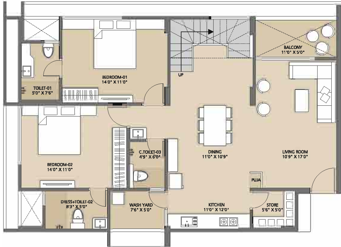
6TH FLOOR BLOCK-D PENTHOUSE (Lower Level)
