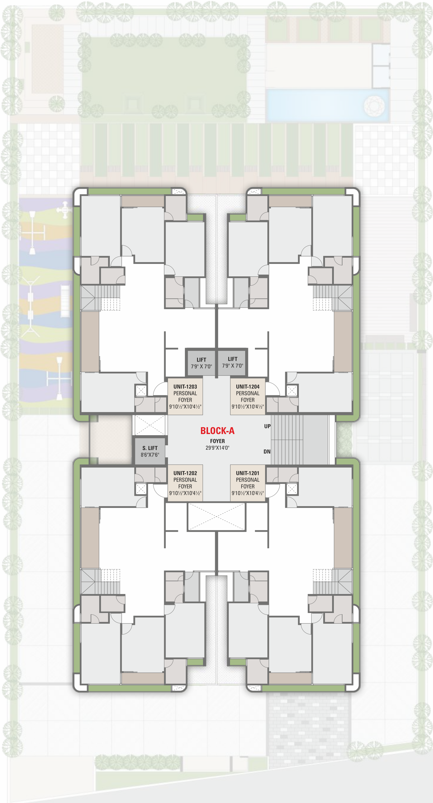
12th FLOOR LAYOUT PLAN ( LOWER PENT HOUSE )
