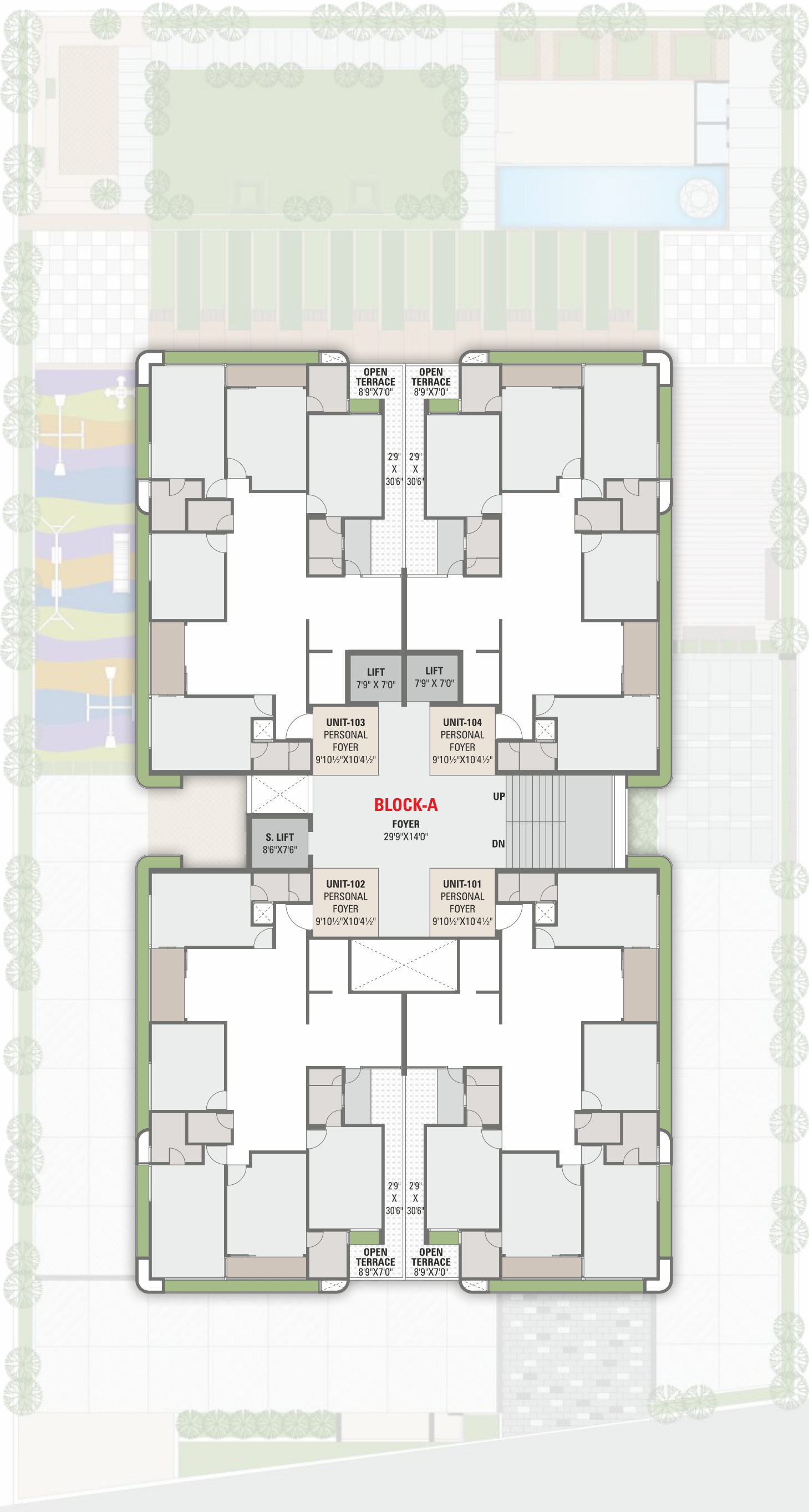
FIRST FLOOR LAYOUT PLAN ✨ ✨
